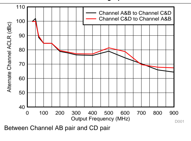
Between Channel AB pair and CD pair Figure 30. Channel Isolation
