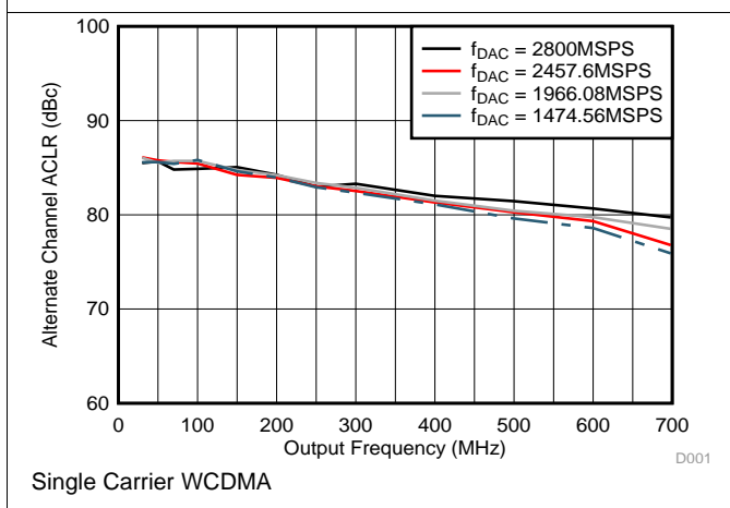
Single Carrier WCDMA Figure 27. ACLR (Alternate Channel) vs Output Frequency Over f_{DAC}
