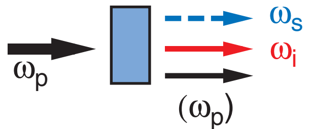
Parametrischer Prozeß \omega_p = \omega_s + \omega_i
